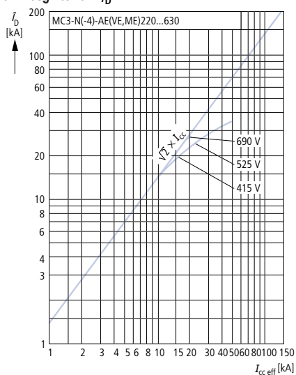
Let-through current i_D
