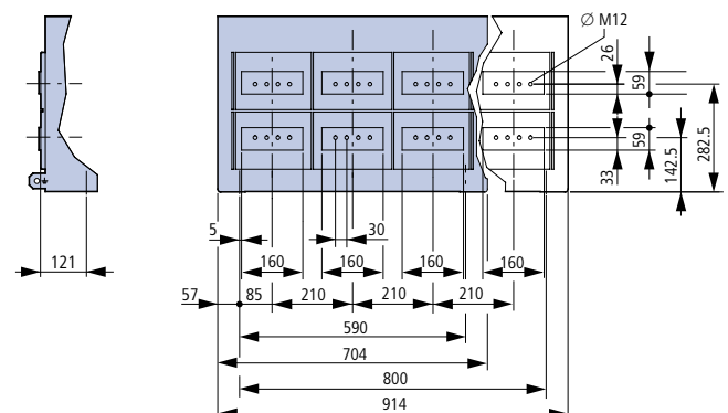
Flange connection
