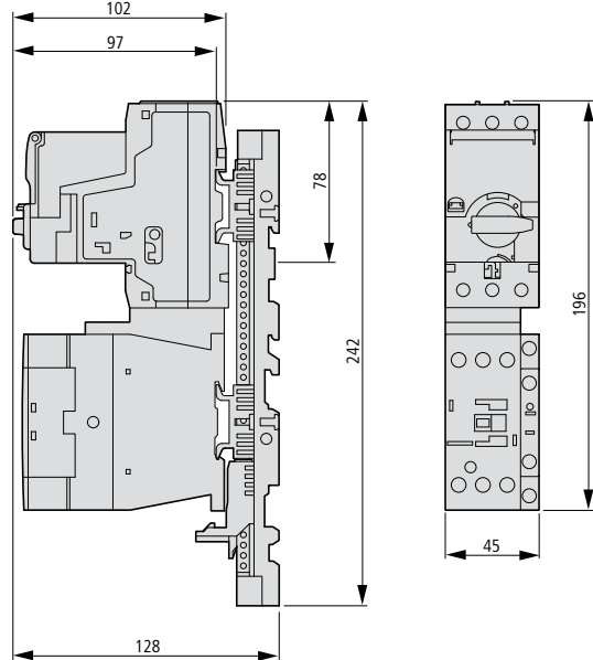
MSC-DE(A)-...-M17[...32]...
