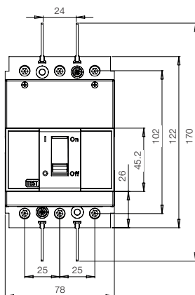
DWB160 B/N / IWB160
