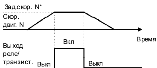
c) N = N^*
