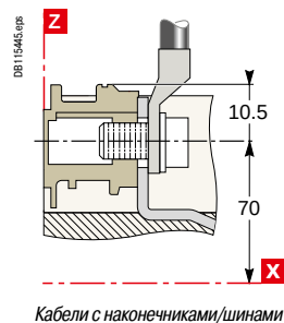
NSX100 – 250 DC
