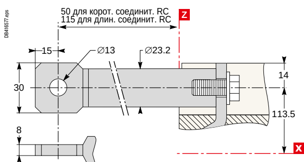
NSX400/630 DC
