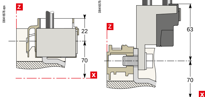
NSX100 – 250 DC
