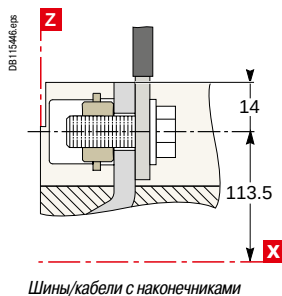
NSX400/630 DC
